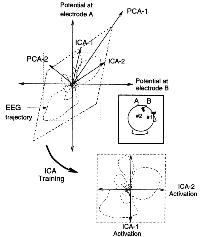
Figure 1. Schematic illustration of independent component analysis (ICA) and principal component analysis (PCA) decompositions of electroencephalogram (EEG) signals (upper left) recorded at two electrodes (A and B), summing the activity of two temporally independent electrooculogram (EOG) (#1) and EEG (#2) sources with differing spatial distributions. PCA finds orthogonal directions of maximum variance in the data. These have no particular relationship to either of the independent components composing the recordings. The ICA algorithm finds the directions of the two axes (ICA-1, ICA-2) by maximizing the entropy of the data transformed linearly to the ICA component axes by a weight matrix and transformed nonlinearly using a compressive nonlinearity (lower right). Maximizing entropy amounts to making the density of the data within the rectangle enclosing the data as uniform as possible, for example, eliminating the empty spaces in the upper left and lower right of the enclosing dotted rectangle (upper left).
