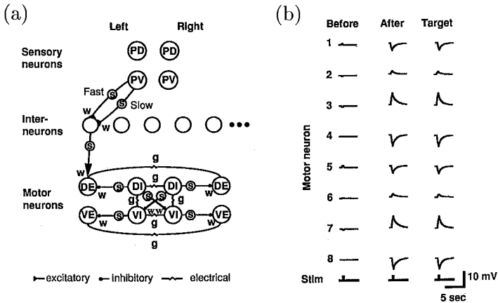
Figure 2: (a) The local bending network model. Four sensory neurons were connected to eight motor neurons via a layer of 10 interneurons. Neurons were represented as single electrical compartments whose voltage varied as a function of time (see text). Known electrical and chemical connections among motor neurons were assigned fixed connection strengths ( g 's and w 's in the motor layer) determined from intracellular recordings. Interneuron input and output connections were adjusted by recurrent backpropagation. Chemical synaptic delays were implemented by inserting s -units between chemically connected pairs of neurons. S -units with different time constants were inserted between sensory and interneurons to account for fast and slow components of synaptic potentials recorded in interneurons (see Fig. 4). (b) Output of the model network in response to simultaneous activation of both PDs (stim). The response of each motor neuron (rows) is shown before and after training. The desired responses from the training set are shown on the right for comparison (target).
