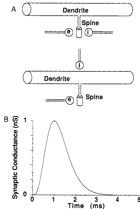
FIG. 1. (A) Geometry of the dendrite and spine for the simulations showing excitation and inhibition on the spine head ( Upper ) and inhibition on the dendritic shaft at the base of the spine ( Lower ). The spine was located in the center of a dendrite with a total length of 300 \mu\text{m} and a diameter of 1 \mu\text{m} ; the spine neck was 1 \mu\text{m} long and 0.1 \mu\text{m} in diameter; the spine head was 0.69 \mu\text{m} long and 0.3 \mu\text{m} in diameter. In the simulations of the electrodiffusion model, sample points in the dendrite were 10 \mu\text{m} apart and the integration time step was 0.1 \mu\text{s} ; in the spine head and neck the spacing was 0.173 \mu\text{m} and 0.167 \mu\text{m} , respectively, and the time steps were 2 \text{ ns} . The model had a total of 41 sample points: 31 in the dendrite, 6 in the spine neck, and 4 in the spine head. In the conventional cable model, only 33 lumped compartments were used (1 for head, 1 for neck, and 31 for dendrite) because of the large space constant. The time step for spine head and neck was 0.1 \mu\text{s} and that for the dendrite was 1 \mu\text{s} . (B) Excitatory and inhibitory synaptic conductance changes were modeled by G(t) = G_M (et/t_{\text{peak}})^4 e^{-4t/t_{\text{peak}}} , where t_{\text{peak}} is the time to reach the peak conductance, G_M . A graph of this expression is shown with t_{\text{peak}} = 1 \text{ ms} , and G_M = 1 \text{ nS} . Parameters used in our simulations were as follows: t_{\text{peak}} = 1 \text{ ms} ; membrane capacitance C_m = 1 \mu\text{F}/\text{cm}^2 ; diffusion coefficients D_K = 1.96 \times 10^{-5} \text{ cm}^2/\text{s} , D_{\text{Na}} = 1.33 \times 10^{-5} \text{ cm}^2/\text{s} , and D_{\text{Cl}} = 2.03 \times 10^{-5} \text{ cm}^2/\text{s} ; resting membrane conductances of unit area g_{K,\text{rest}} = 1.95 \times 10^{-4} \text{ S}\cdot\text{cm}^2 , g_{\text{Na},\text{rest}} = 1.63 \times 10^{-5} \text{ S}\cdot\text{cm}^2 and g_{\text{Cl},\text{rest}} = 3.89 \times 10^{-5} \text{ S}\cdot\text{cm}^2 ; initial intracellular concentrations n_{K,0} = 140 \text{ mM} , n_{\text{Na},0} = 12 \text{ mM} , and n_{\text{Cl},0} = 5.5 \text{ mM} ; extracellular concentrations n_{K,\text{out}} = 4 \text{ mM} , n_{\text{Na},\text{out}} = 145 \text{ mM} , and n_{\text{Cl},\text{out}} = 120 \text{ mM} . With this set of parameters, the resting membrane potential was -78 \text{ mV} . The Nernst potentials for \text{K}^+ , \text{Na}^+ , and \text{Cl}^- were -90 , 63 , and -78 \text{ mV} , respectively. Total membrane resistivity R_m was 4000 \Omega\cdot\text{cm}^2 . Total cytoplasmic resistivity R_i at rest was calculated (8) to be 87 \Omega\cdot\text{cm} . Total surface area of the spine head was 0.65 \mu\text{m}^2 . Some of these parameters were varied as explained in the relevant figures and tables. The sources for these parameters are given in ref. 8.
