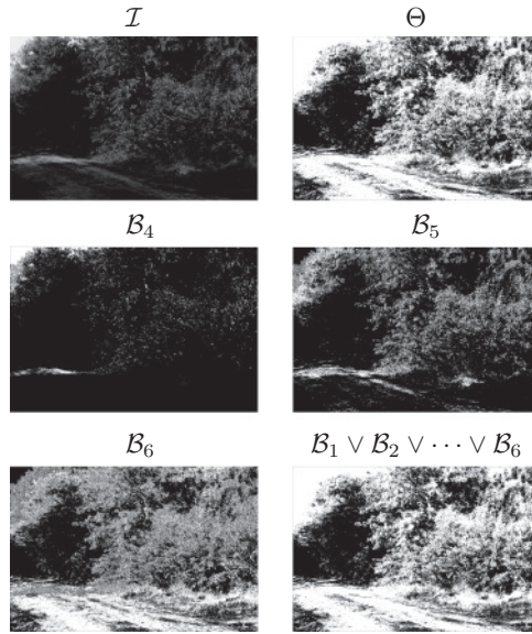
Figure 1: Example of an image \mathcal{I} from the van Hateren database. Its median thresholded image \Theta and the bit planes \{\mathcal{B}_4, \mathcal{B}_5, \mathcal{B}_6\} are shown. \theta(\mathcal{I} - \text{median}(\mathcal{I})) \simeq \mathcal{B}_1 \vee \mathcal{B}_2 \vee \dots \vee \mathcal{B}_6 is also demonstrated, which is a good approximation for this example as \mu = L - \log_2(\text{median}(I)) = 5.9447 is close to 6.
