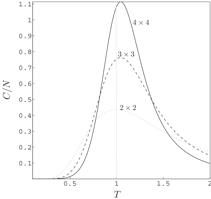
Figure 2: The specific heat curves C/N calculated the ensemble \Theta = \theta(\mathcal{I} - \text{median}(\mathcal{I})) . They are plotted versus temperature T for systems of size N = \{2 \times 2, 3 \times 3, 4 \times 4\} . The ensemble \Theta is at T = 1 .
