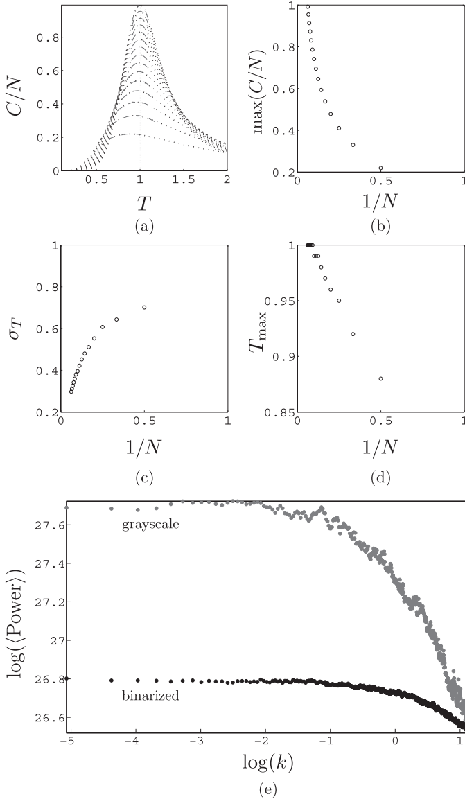
Figure 3: Studying 1D samples from the ensemble \Theta for systems of linear size N = \{2, 3, \dots, 16\} . (a) C/N is plotted versus T . The dashed curves are the gaussian fit around the peak. (b) Finite size scaling. The peak of C/N is plotted versus 1/N . (c) Here the width \sigma_T (obtained from the gaussian fit near the peak) is plotted versus 1/N . (d) The location of the peak is plotted versus 1/N . Unlike the curves in panels b and c, it saturates in the large N limit. (e) The power spectrum of 1D stripes with 1000 pixels before (in gray) and after binarization (in black) are given. The data points for binarized samples are shifted up by 14.7.
